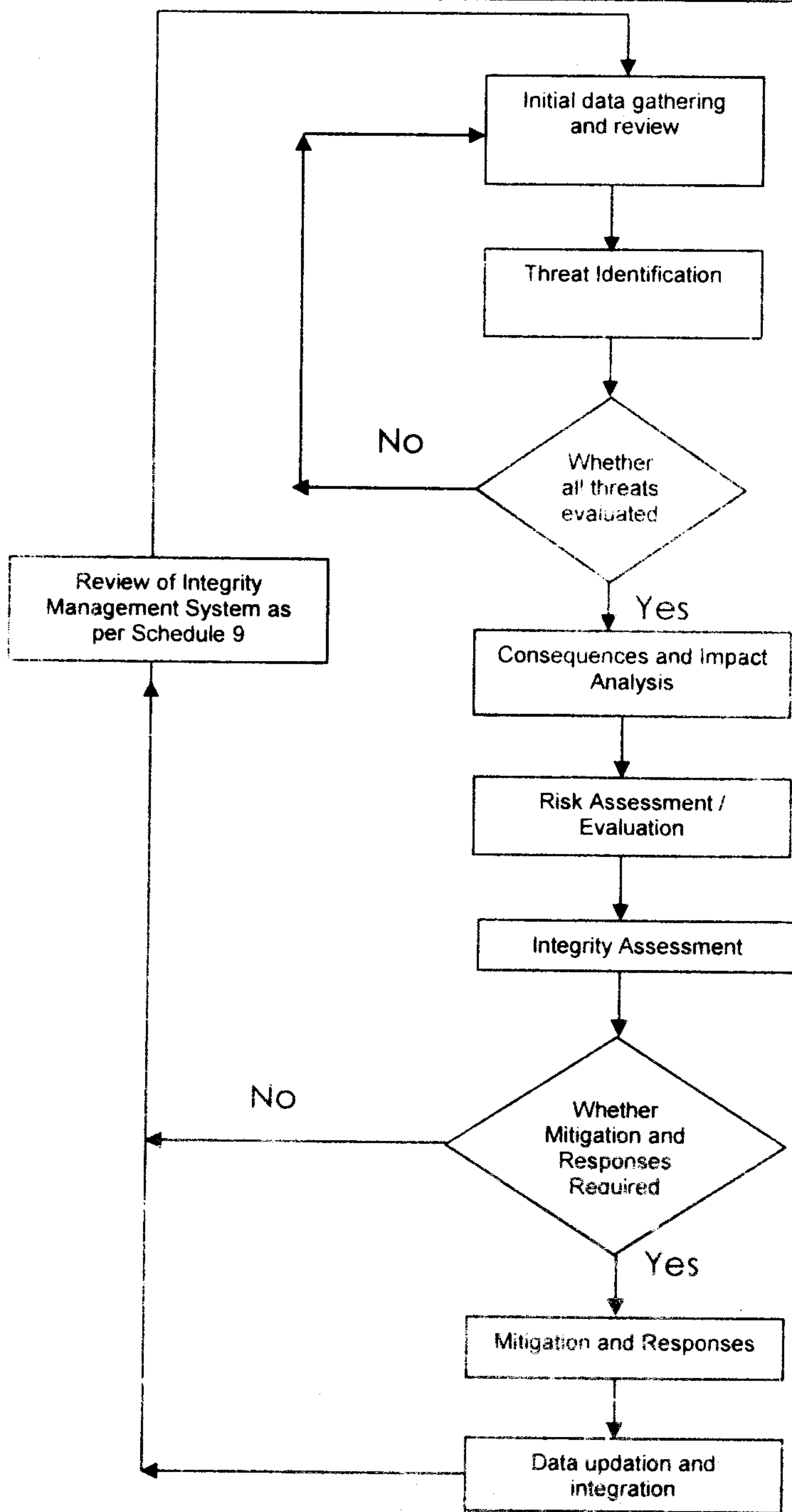
Figure-1: Pipeline Integrity Management Plan - Flow Diagram
